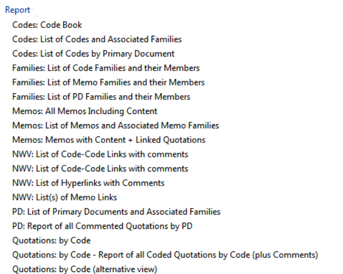
Figure 354: Available Reports
