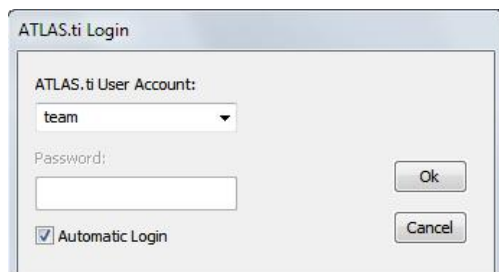
Figure 107: Login Window
