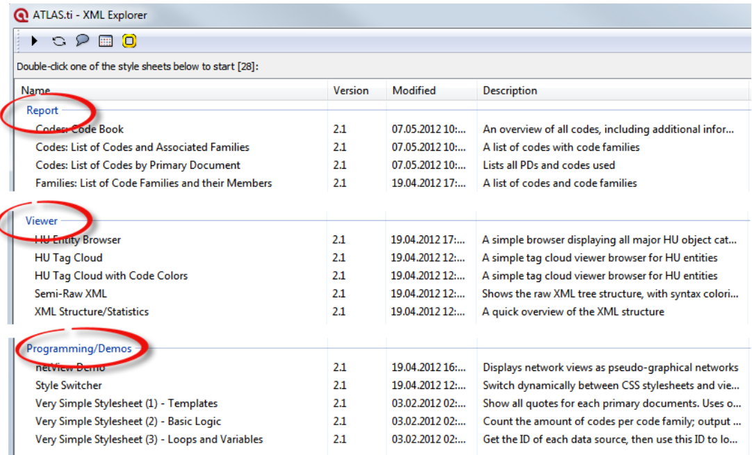
Figure 353: XML Explorer
