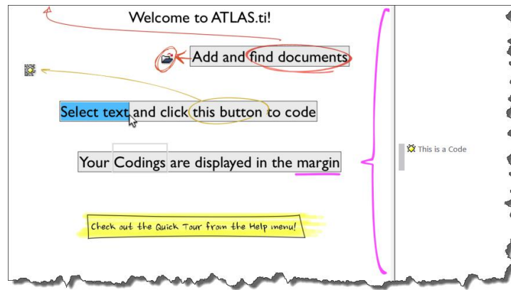
Figure 48: Welcome document
