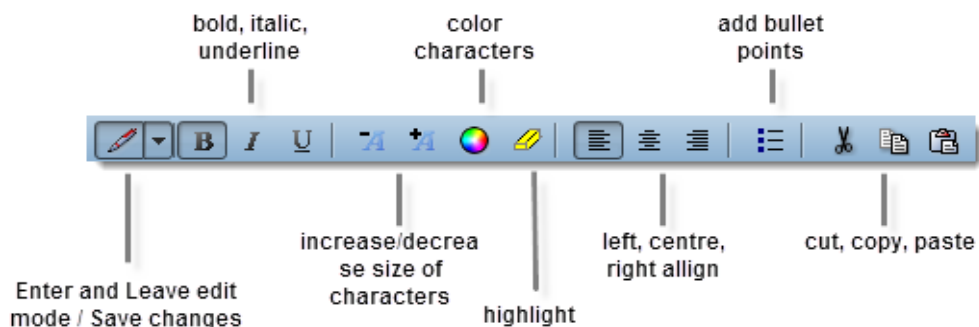
Figure 174: Edit toolbar
