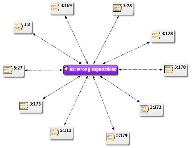
Figure 264: Code-quotations links
