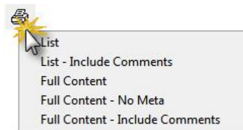
Figure 216: Output options
