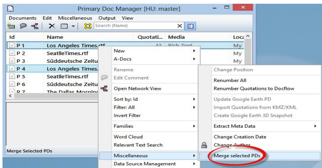
Figure 117: Merge duplicates
