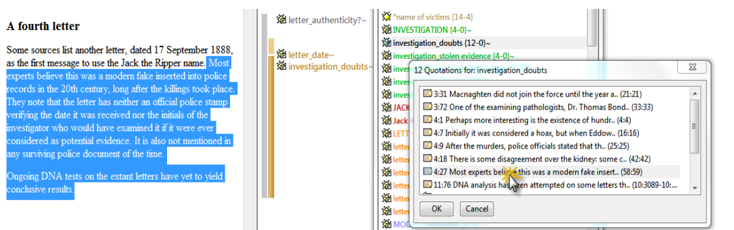
Figure 163: Simple retrieval
