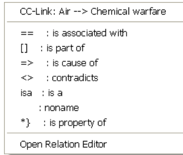
Figure 300: Relations
