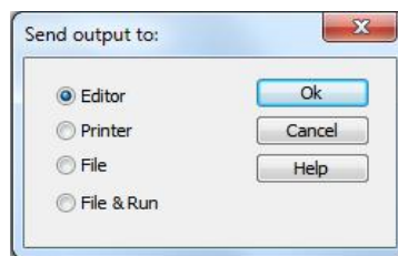
Figure 164: Output options
