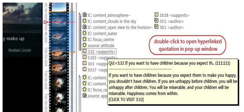
Figure 320: Traversing hyperlinks
