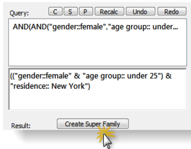
Figure 231: Clicking a more complex query - step 3
