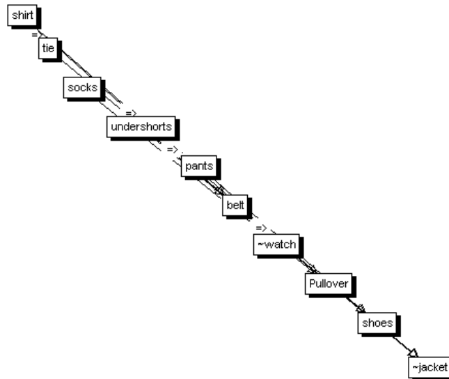
Figure 296: Topological sort always results in a linear, diagonal placement of the nodes
