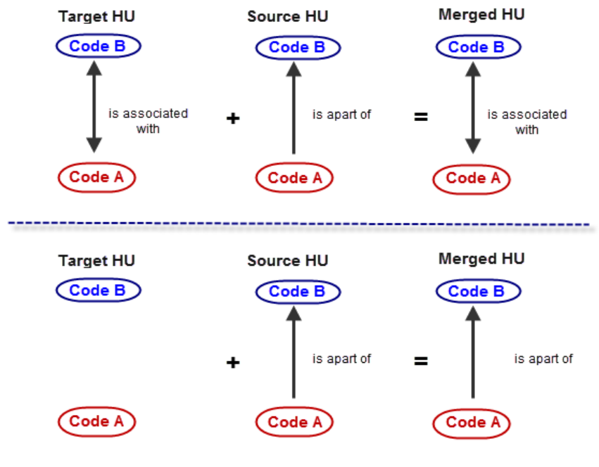
Figure 119: Merging HUs: Link resolution - The link between Code A and Code B in the target HU survives the merge process.
