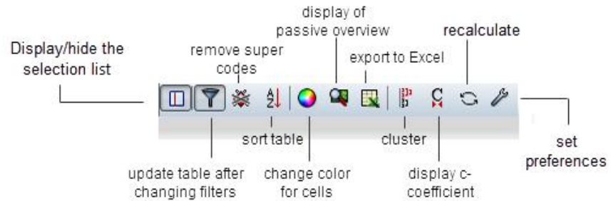
Figure 242: The Codes Co-occurrence Table toolbar
