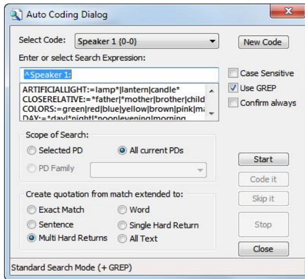
Figure 170: Auto Coding Dialog window
