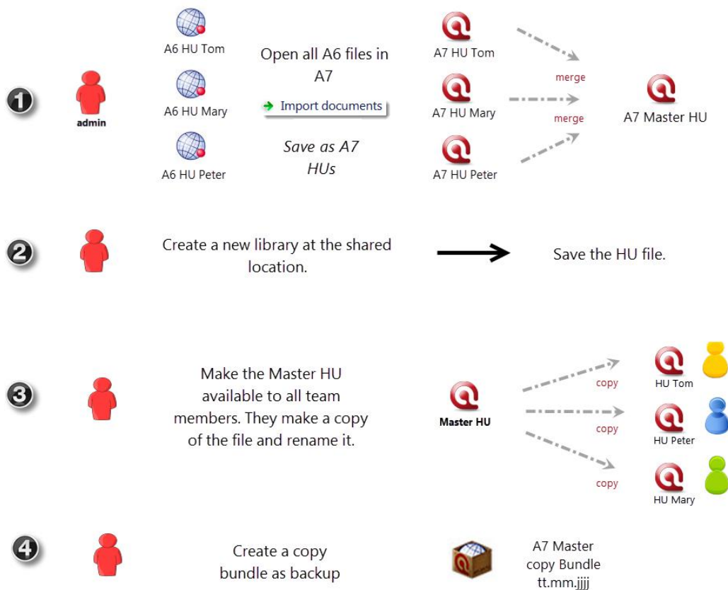
Figure 103: Work flow for team project migration if a common data set is stored at a shared location
