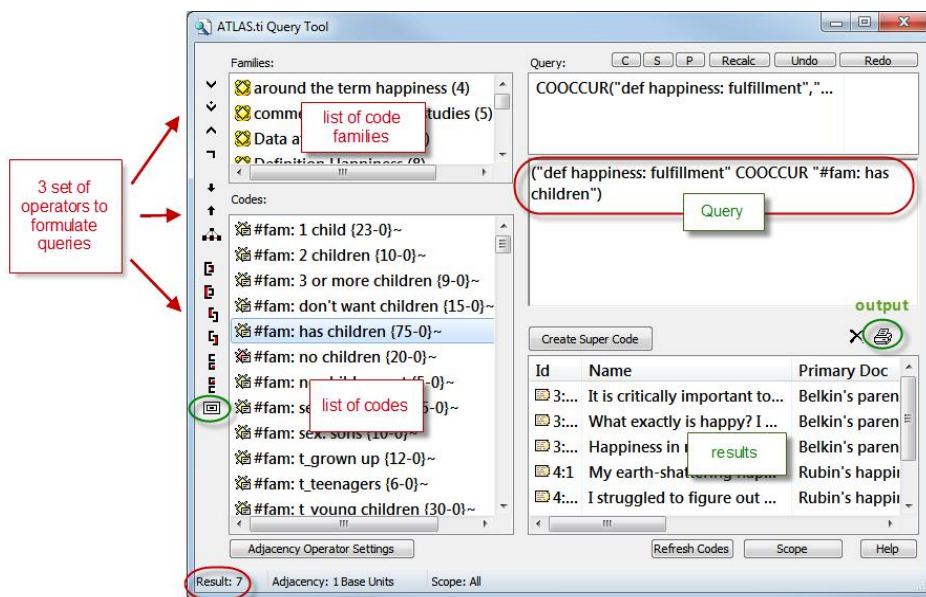
Figure 218: Query tool window
