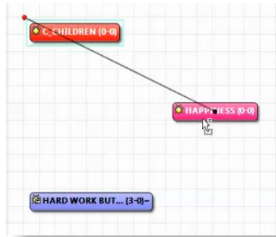
Figure 272: Linking nodes
