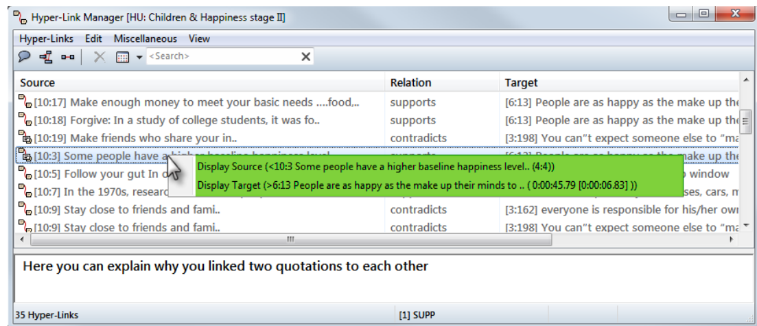
Figure 321: Hyperlink Manager
