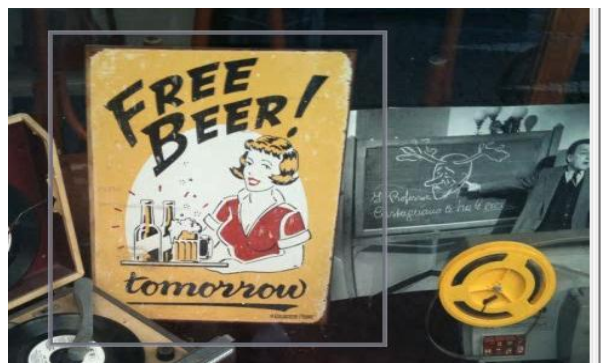
Figure 125: Graphical quotation
