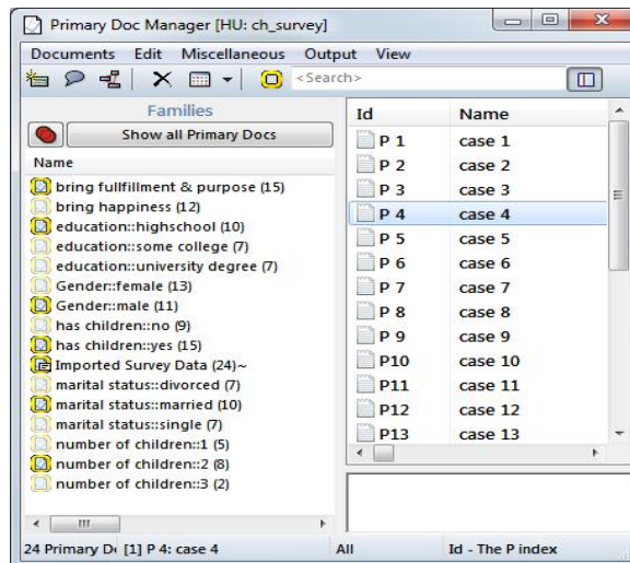
Figure 86: P-Docs Manager with imported survey data and the corresponding families
