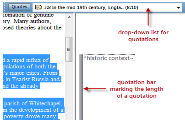
Figure 123: Quotation reference
