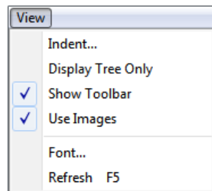
Figure 335: View menu
