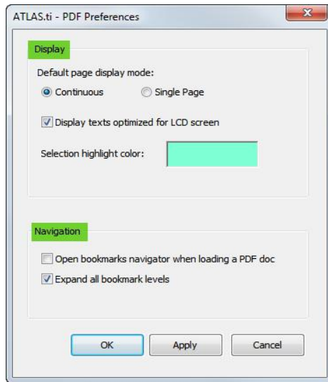
Figure 398: PDF Preferences
