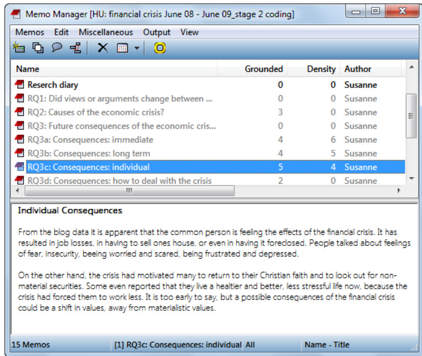
Figure 33: Memo Manager
