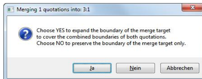
Figure 200: Merging quotations
